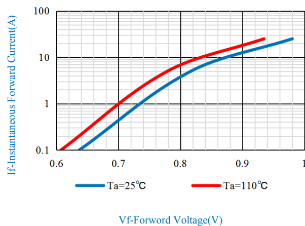
Fig.2-Typical Instantaneous Forward
