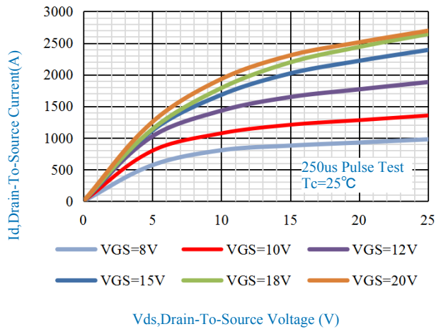
Fig.1-Output Characteristic@Tj=25°C
