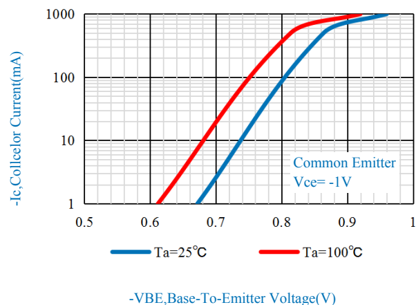
Fig.6-Base-To-Emitter Voltage Characteristics
