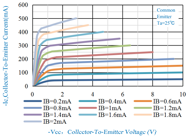
Fig.1-Static Characteristics
