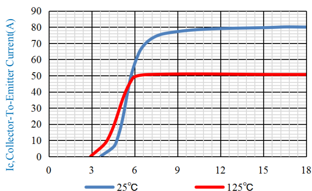
Fig.3-Transfer Characteristic
