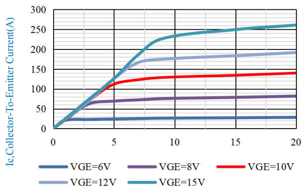
Fig.1-Output Characteristic@ T_j = 25^\circ\text{C}
