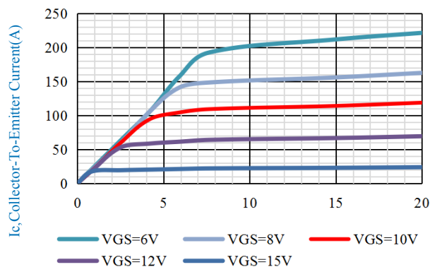
Fig.2-Output Characteristic@ T_j = 175^\circ\text{C}
