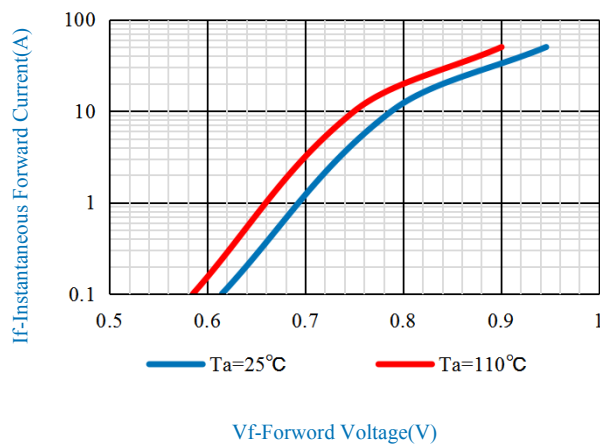
Fig.2-Typical Instantaneous Forward
