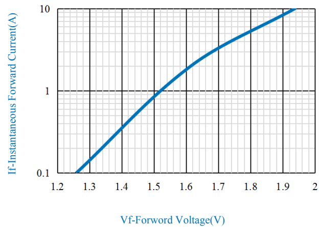
Fig.2-Typical Instantaneous Forward
