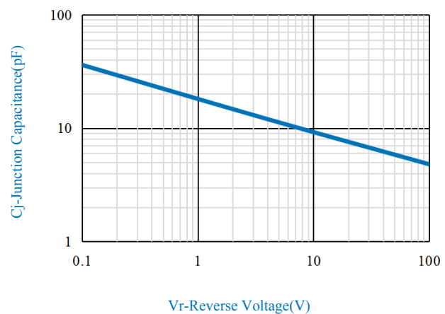
Fig.4-Typical Junction Capacitance
