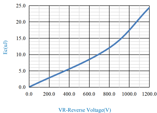
Fig.8-Capacitance Stored Energy
