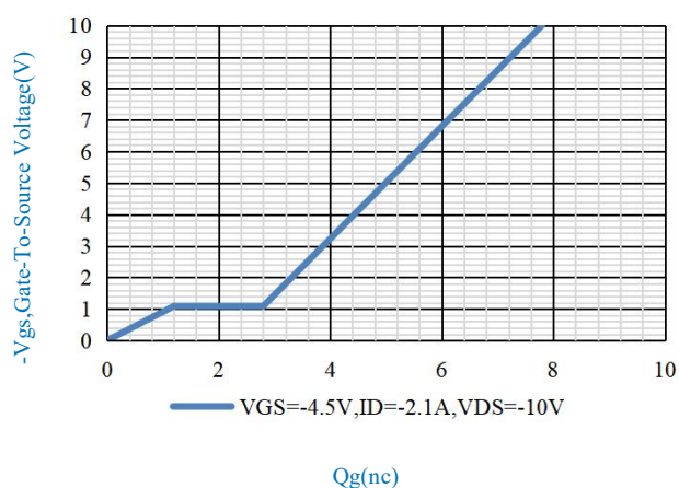
Fig.11-Gate Charge Waveform
