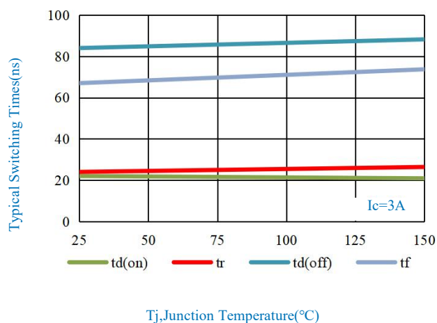
Fig.7-Typical Switching Times Vs. Junction Temperature
