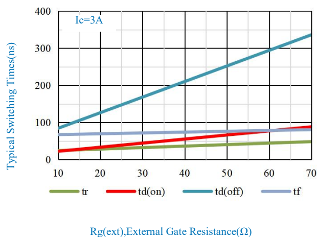
Fig.8-Typical Switching Times Vs. External Gate Resistance
