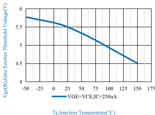
Fig.4-Gate Emitter Threshold Voltage Vs. Junction Temperature
