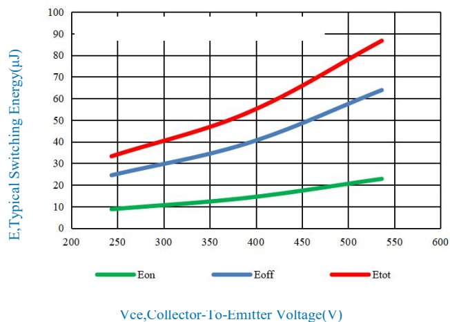
Fig.12-Typical Switching Energy Vs. Collector-To-Emitter Voltage
