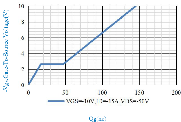
Fig.11-Gate Charge Waveform
