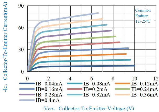
Fig.1-Static Characteristics
