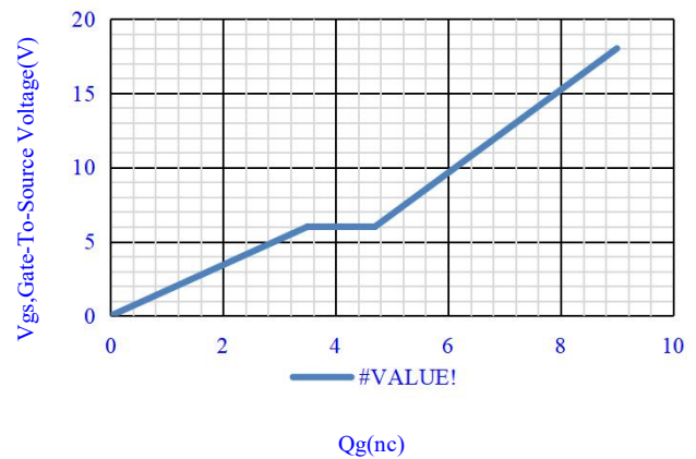
Fig.16-Gate Charge Waveform
