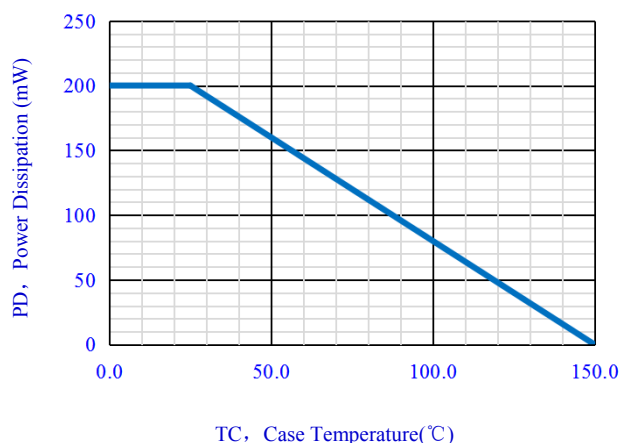
Fig.6-Maximum Power Dissipation vs. Case Temperature
