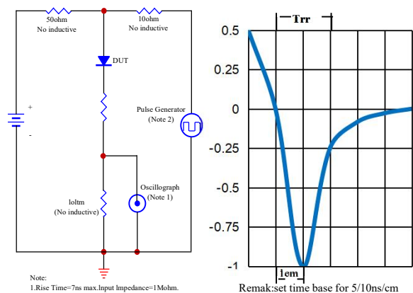
Fig.6-REVERSE RECOVERY TIME CHARACTERISTIC AND TEST CIRCUIT
