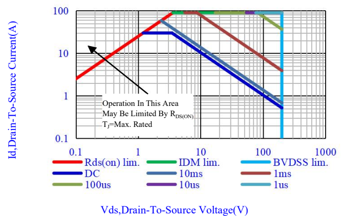
Fig.12-Maximum Safe Operating Area(SOA)
