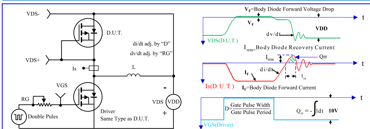
Fig.16- Diode Recovery Test Circuit & Waveform
