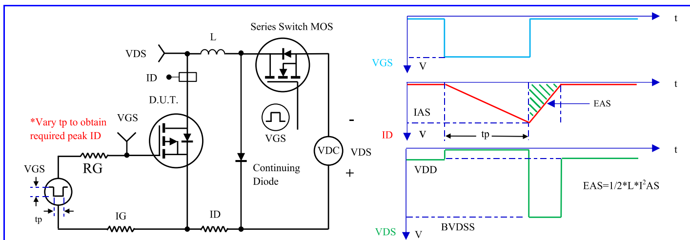
Fig.15- Unclamped Inductive Switching (UIS) Test Circuit & Waveform
