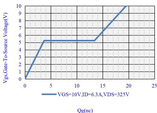
Fig.10-Gate Charge Waveform
