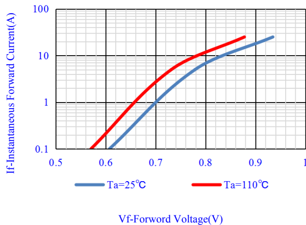
Fig.2-Typical Instantaneous Forward
