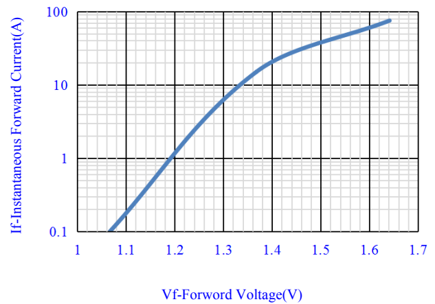
Fig.2-Typical Instantaneous Forward
