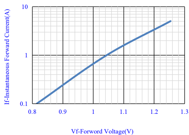
Fig.2-Typical Instantaneous Forward
