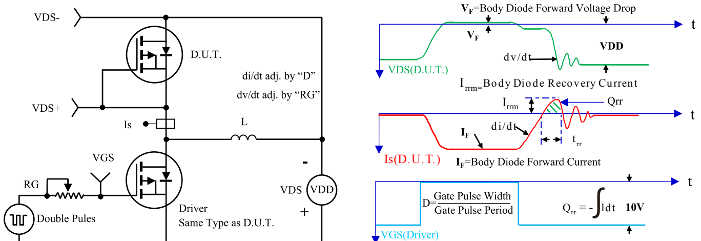
Fig.17- Diode Recovery Test Circuit & Waveform
