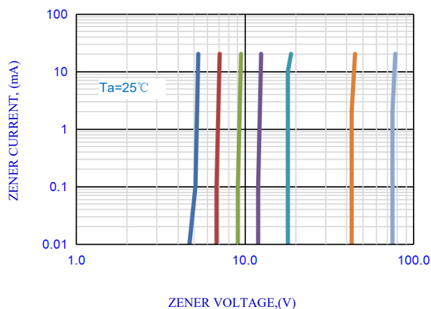
Fig.5-ZENER BREAKDOWN CHARACTERISTICS
