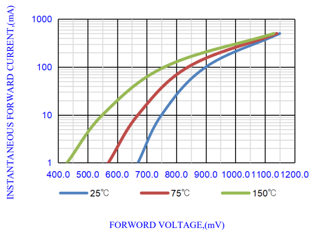
Fig.2- Forward characteristics
