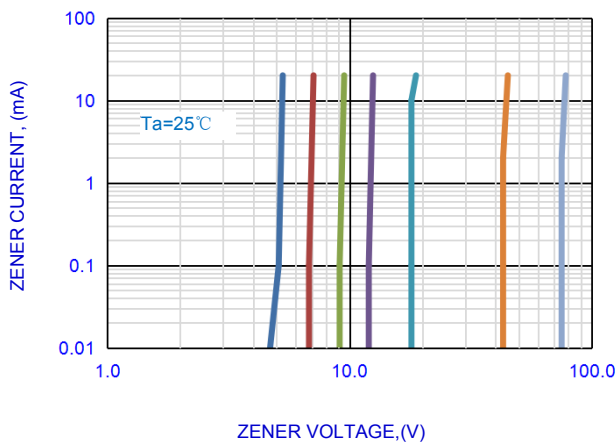
Fig.5-ZENER BREAKDOWN CHARACTERISTICS
