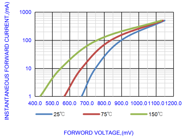
Fig.2- Forward characteristics
