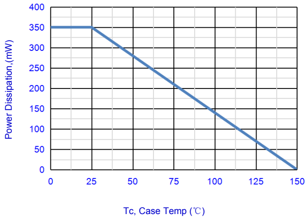
Fig.1-POWER DISSIPATION VS. AMBIENT TEMP.
