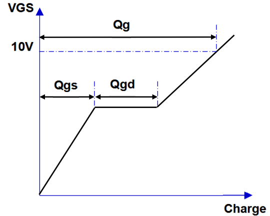
Fig.15- Gate Charge Test Circuit & Waveform
