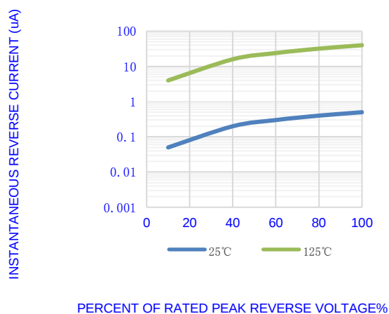
Fig.3-TYPICAL REVERSE CHARACTERISTICS
