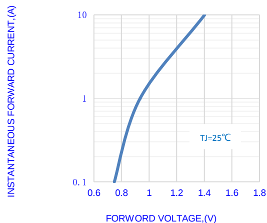
Fig.2-TYPICAL INSTANTANEOUS FORWARD
