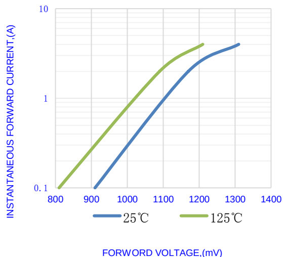
Fig.2-TYPICAL INSTANTANEOUS FORWARD
