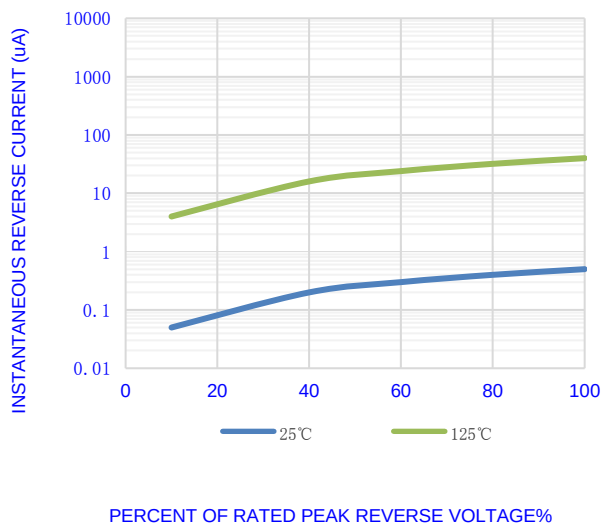
Fig.3-TYPICAL REVERSE CHARACTERISTICS
