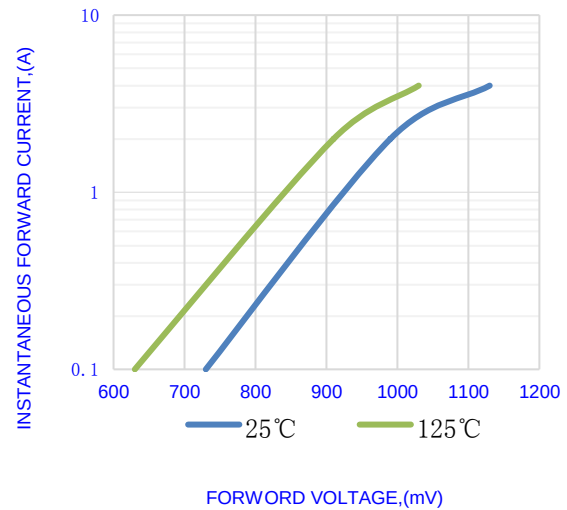
Fig.2-TYPICAL INSTANTANEOUS FORWARD
